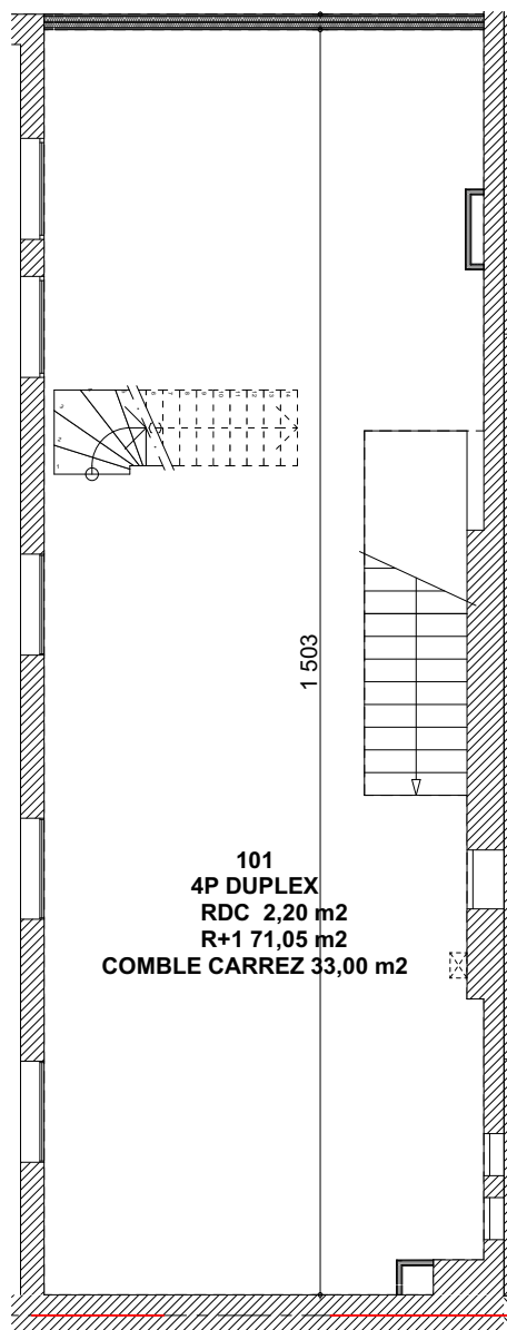
PLAN R+1
