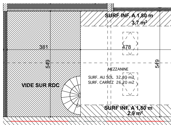
PLAN R+1
