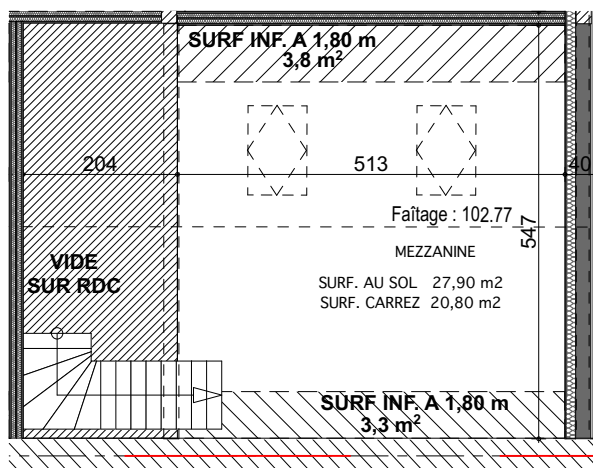
PLAN R+1
