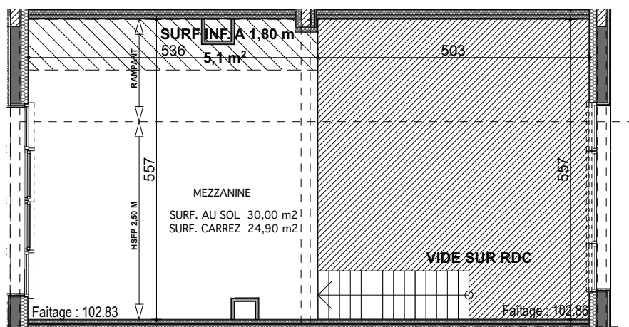
PLAN R+1
